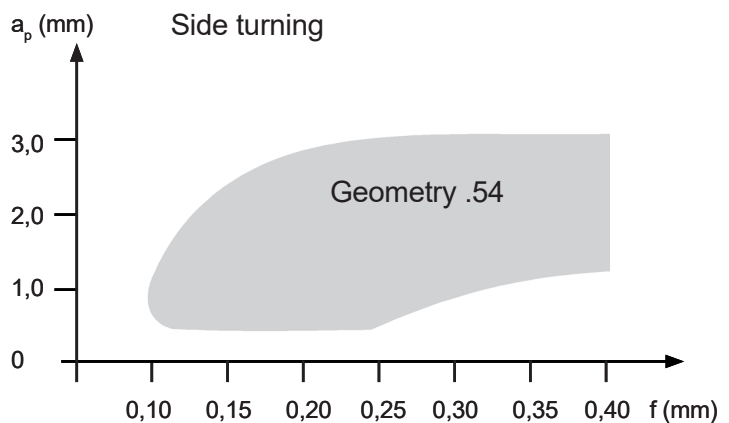
Chip control graph S224.0500.54 material 16MnCr5
